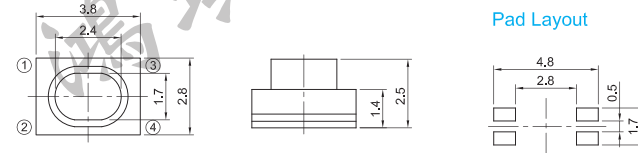
Pad Layout
