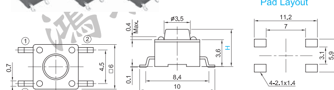
Pad Layout
