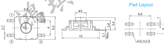
Pad Layout
