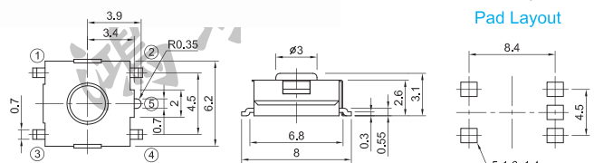
Pad Layout
