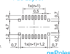
Pad Layout
